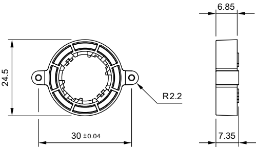
14 Switching element PCB mounting illuminative page 21
