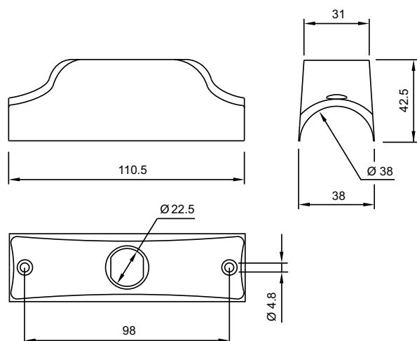
19 Housing, pole mounting 38 mm dia. page 25
