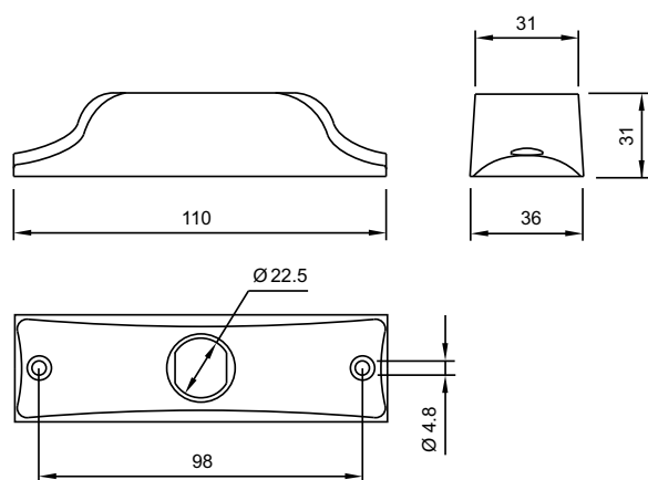
20 Housing, wall mounting page 26
